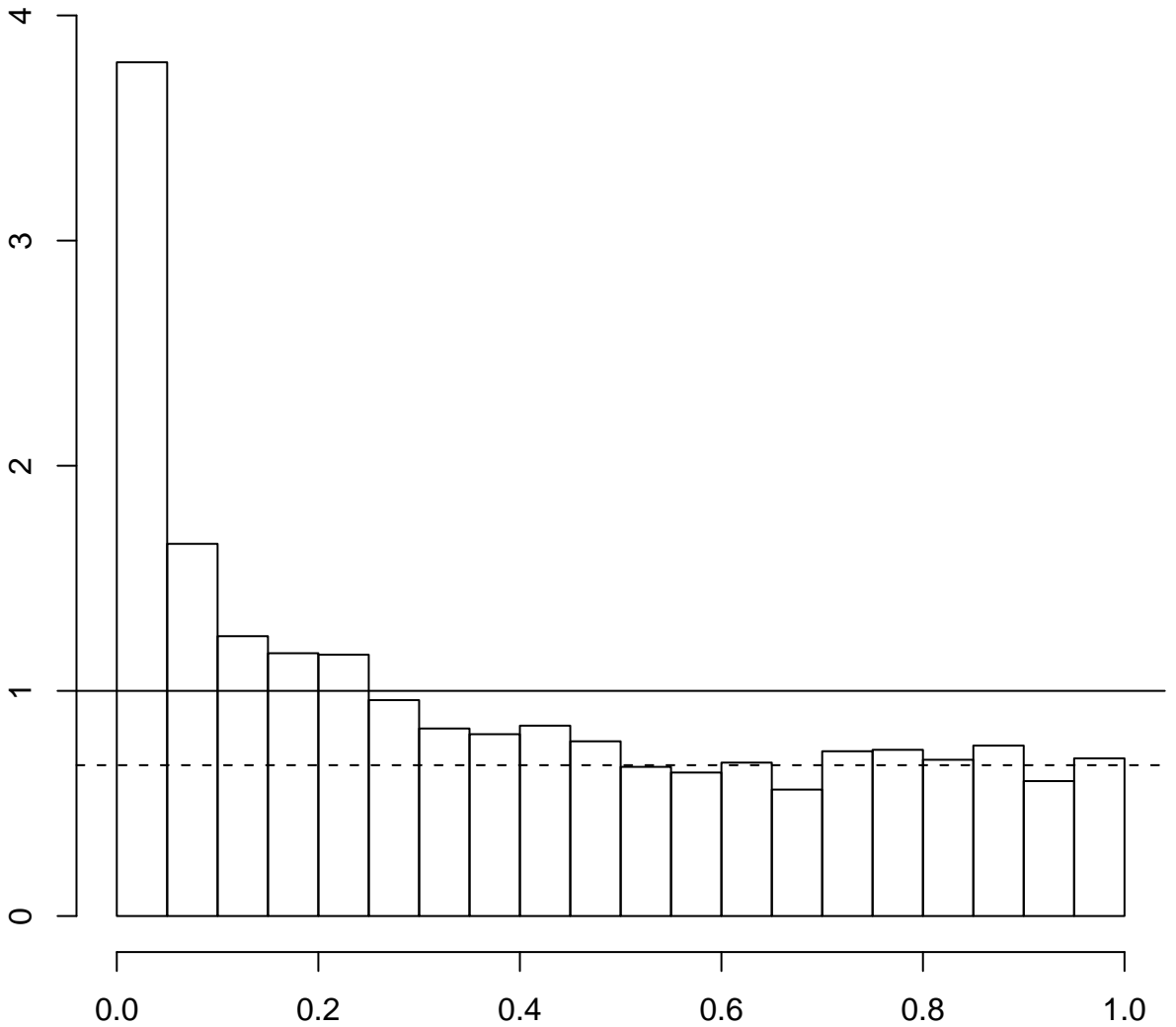
Density of observed p-values
